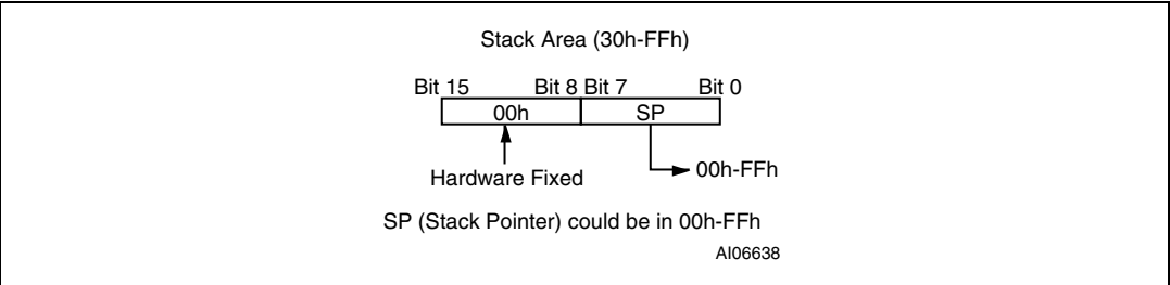
Figure 7. Stack pointer
